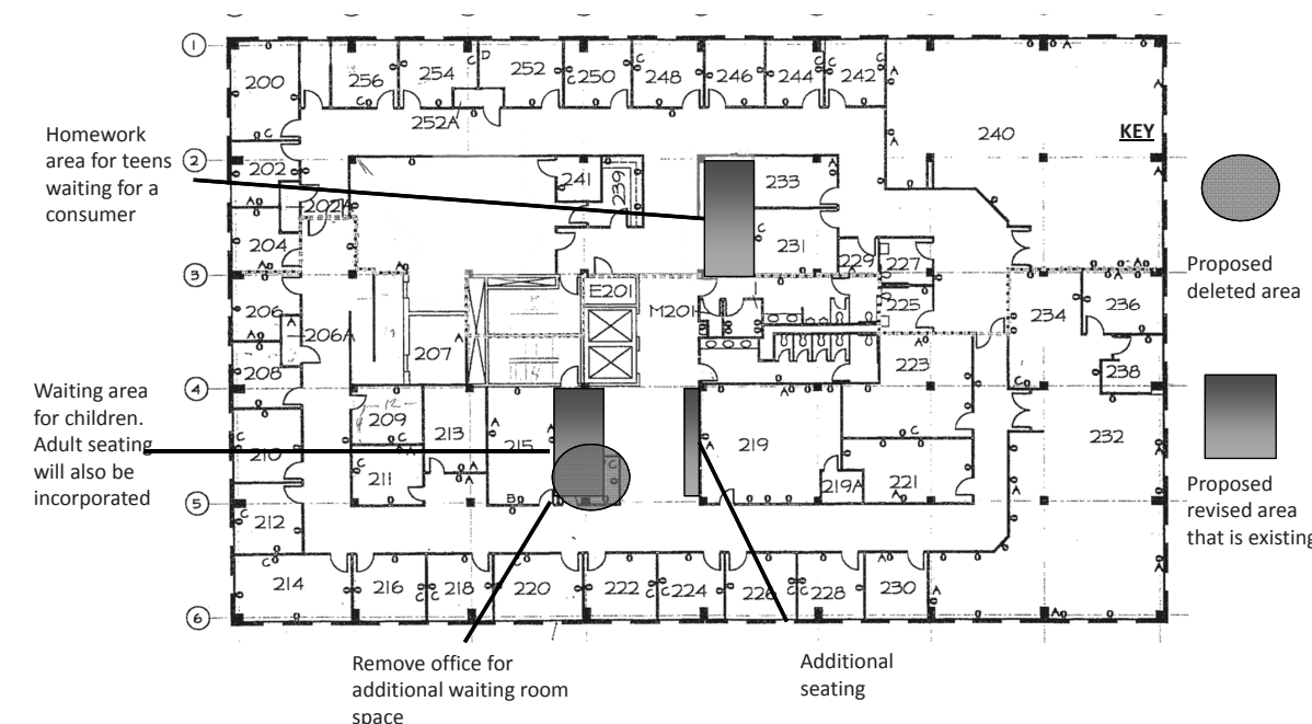
Existing Floorplan
