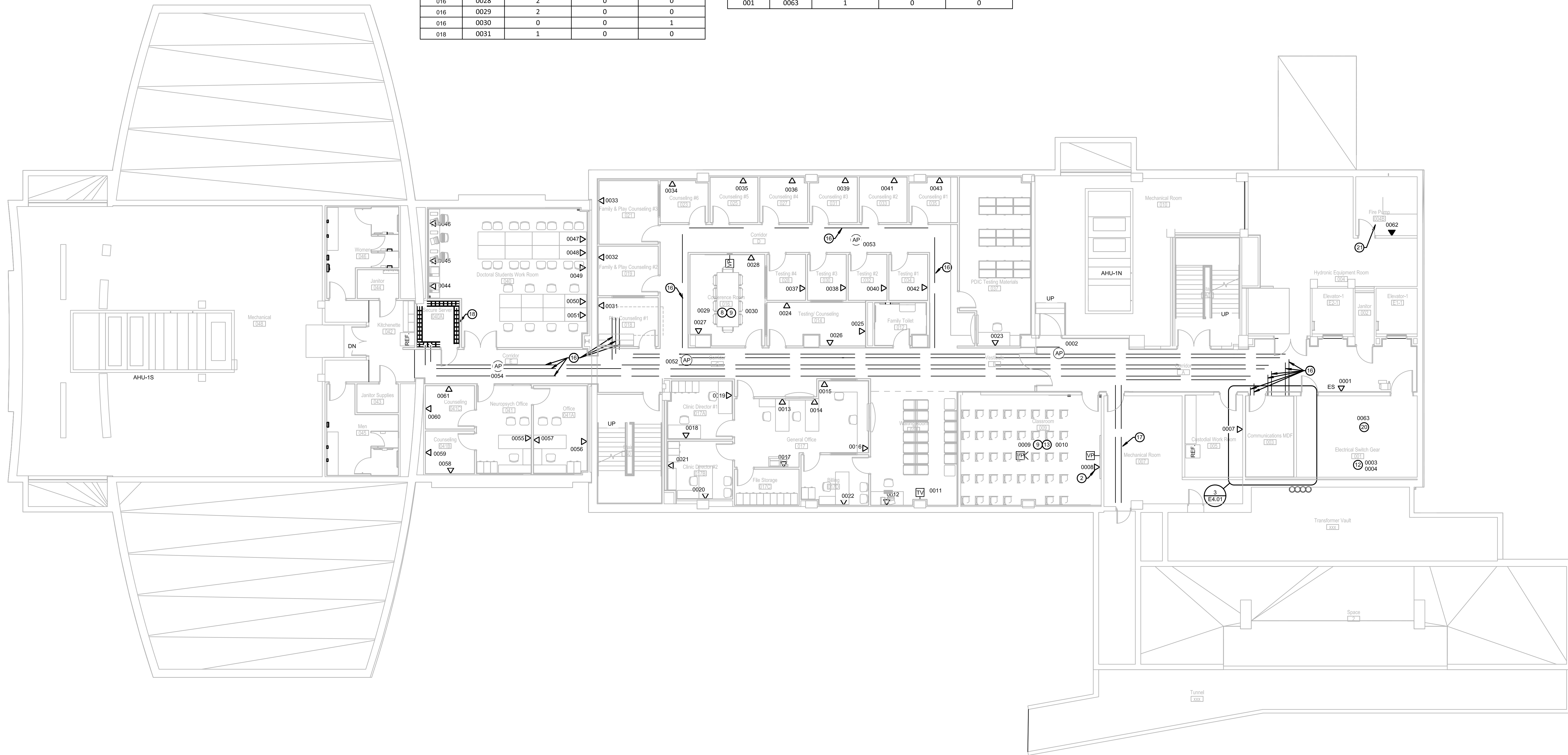
Lower Level Systems Plan Scale: 1/8" = 1'-0"
